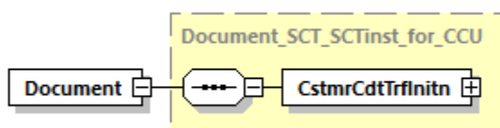
Abbildung 139: pain.001.001.09, Document
