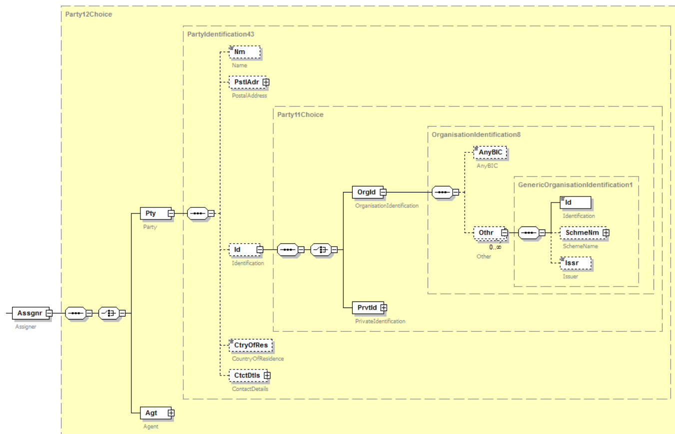
Abbildung 155: camt.055.001.05, Assgnr
