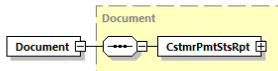
Abbildung 85: pain.002.001.10, Document
