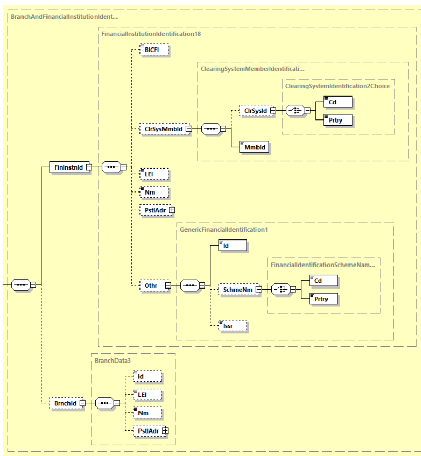
Abbildung 96: pain.002.001.10, BranchAndFinancialInstitutionIdentification6
